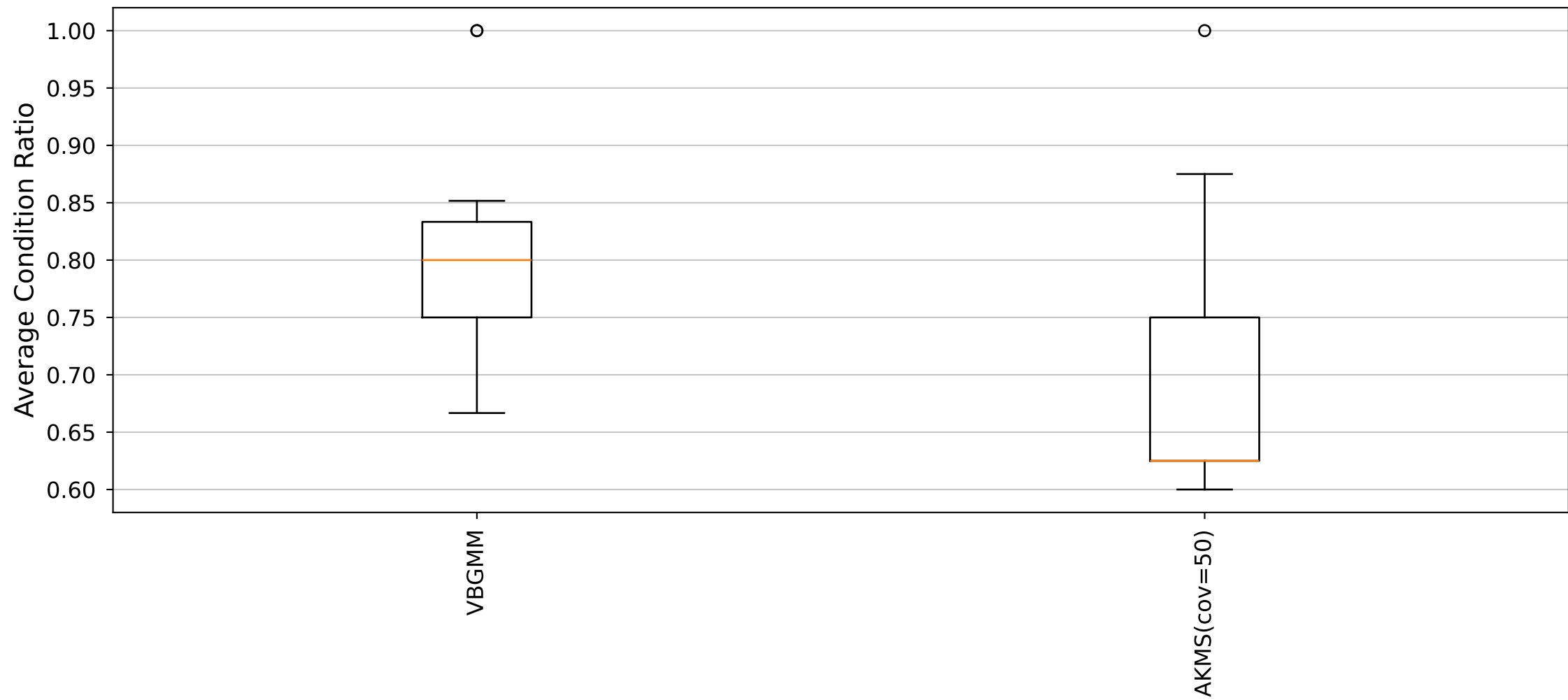
YARA Rules Average Condition Ratio Distribution (Cluster10_Size10 dataset)
